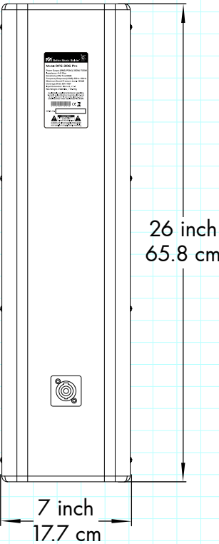
Rear View
